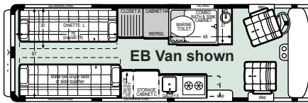
(O) Options • Swivels for Cab Captain's Seats
