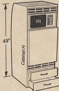
CABINET H Will accommodate Std. 3 CF refrigerator.
