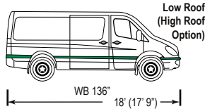
RB (REGULAR BODY) 1500 GVWR 8,550
