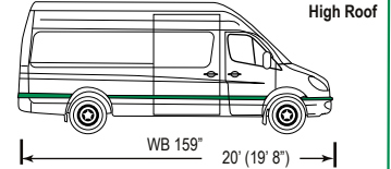
EB (EXTENDED BODY) 3500 GVWR 9,350
